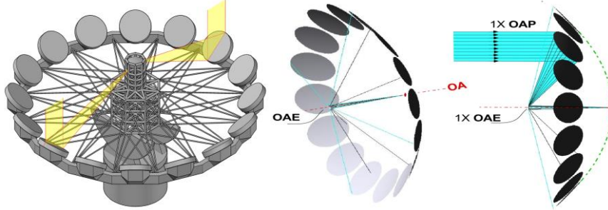
Figure 4. ELF Gregorian-focus off-axis parabolic optical configuration.
