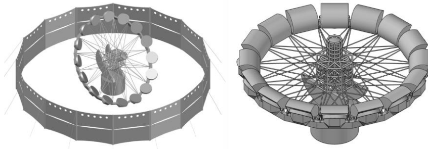
Figure 5. ELF Mechanical enclosure concepts: wind fence (left) and mirror covers (right).
